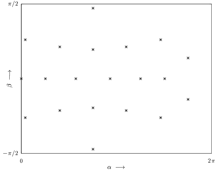
FIGURE 2. Final configuration, as in Figure 1, where the Fekete points are given in the \{\alpha, \beta\} -plane. A rotation has been applied such that (11) is fulfilled.
